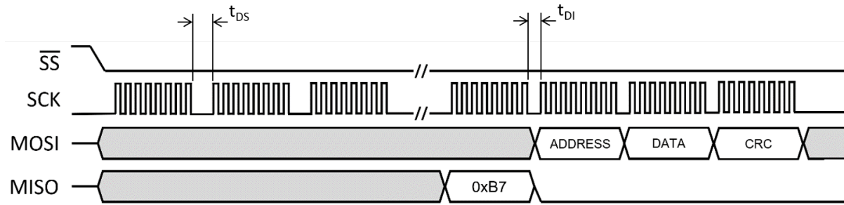
Figure 17. SPI Command Polling Timing Diagram
