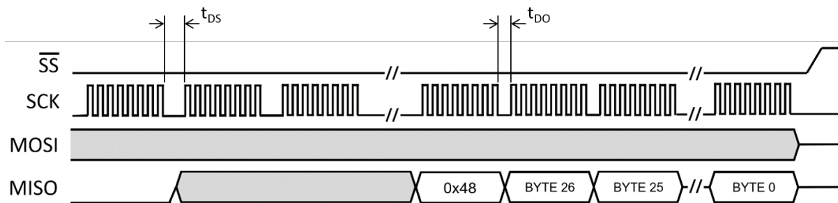
Figure 18. SPI Response Polling Timing Diagram
